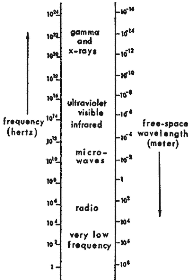
Figure 1. The Electromagnetic Spectrum
